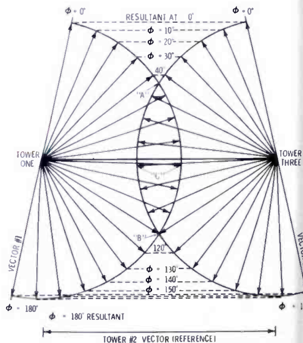
VECTOR PLOT OF TABLE 1 NULLS OCCUR AT POINT OF OVERLAP
